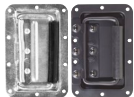
No. 30000900 .....silver No. 30000920 .....black ROADINGER Hinged case handle • Sprung handle • Weight approx. 350 g • Cut-out 130 x 73 mm • Mounting holes: d=5.0 mm
