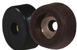
No. 30001200 .....large, steel-reinforced No. 30001202 ..... 25 x 25 mm No. 3000130A .....small, with steel ring ROADINGER Rubber foot • With steel disk insert • Diameter: 38 mm • Height: 20 mm • Weight: approx. 30 g • Mounting hole: d= 5.5 mm
