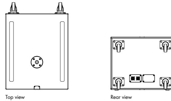
B6-SUB cabinet dimensions in mm [inch]
