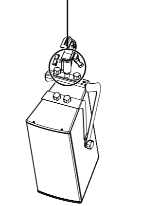
Yi7P/Yi10P with Z5399 YP Mounting bracket Z5010 TV Spigot with fixing plate Z5012 Pipe clamp
