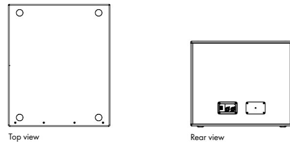
Bi6-SUB cabinet dimensions in mm [inch]
