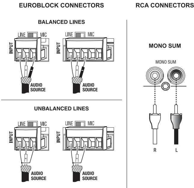
Figure 2.4.1 Input Wiring
